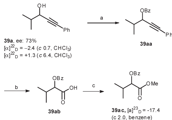
Scheme 2 The synthesis of 39ac to confirm the absolute configuration of 39a . Reagents and conditions: (a) BzCl, Et 3 N, DCM; (b) OsO 4 , NaIO 4 , HMTA, THF/H 2 O; (c) catalytic conc. H 2 SO 4 , MeOH.
