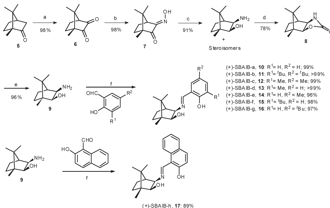
Scheme 1 The synthesis of SBAIB Ligands. Reagents and conditions : (a) SeO 2 , Ac 2 O, reflux, 17 h, 98%; (b) H 2 NOH.HCl, NaOAc, EtOH/H 2 O, reflux, 15 min, 98%; (c) LiAlH 4 , THF, reflux, 20 h, 91%; (d) (Cl 3 CO) 2 CO, 6 M NaOH, DCM, -5 °C, 1 h then rt, 2.5 h, 78%; (e) 3 M NaOH, EtOH/H 2 O, reflux, 6 h, 96%; (f) Anhy. Na 2 SO 4 , EtOH/DCM, reflux, 12 h.
