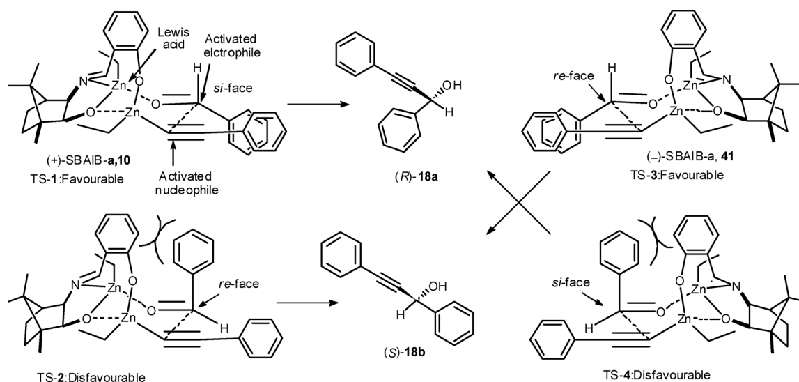
Fig. 3 The proposed mechanism.
