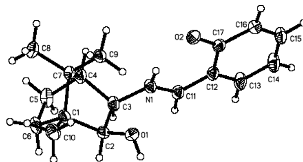
Fig. 2 X-ray crystallographic structures of (+)-SBAIB-a, 10 (CCDC 823886f).
