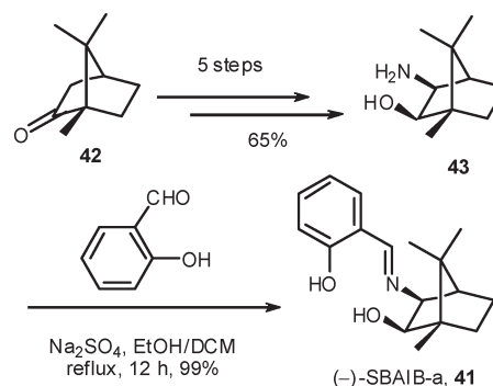
Scheme 4 The synthesis of (–)-SBAIB-a, 41 from ( 1S )-camphor.
