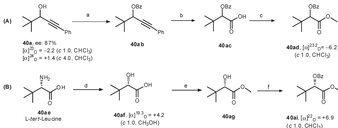
Scheme 3 Syntheses of 40ad and 40ai to confirm the absolute configuration of 40a . Reagents and conditions: (a) BzCl, Et 3 N, DCM; (b) OsO 4 , NaIO 4 , HMTA, THF/H 2 O; (c) catalytic conc. H 2 SO 4 MeOH; (d) 2 M NaNO 2 , 2 N H 2 SO 4 ; (e) catalytic conc. H 2 SO 4 ; (f) BzCl, Et 3 N, DMAP, DCM.
