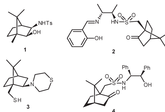
Fig. 1 Camphor-based ligands for enantioselective alkylation to aldehydes.
